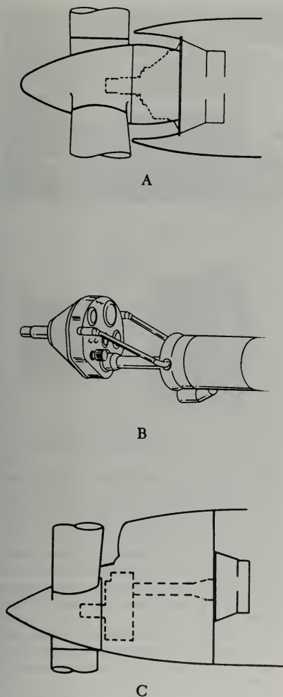
FIGURE 2-24. Turboprop compressor inlets.
